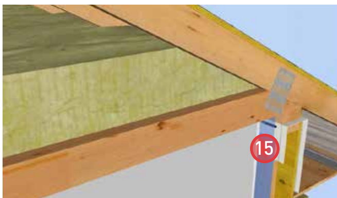
15. Install ROXUL® COMFORTBATT® in the attic space.
