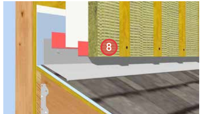
8. Install ROXUL® COMFORTBOARD™ 80 and secure in place with strapping. Provide bugscreens at the top and bottom of the strapping.
