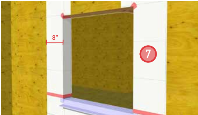
7. Install sheathing membrane pre-strips at the jambs and extend onto face of wall a minimum of 8". Lap the sheathing membrane over the self-adhered membrane at the corners and seal the leading edges with sheathing tape.
