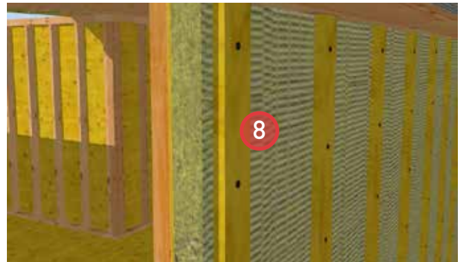
8. Install ROXUL® COMFORTBOARD™ 80 and strapping. Provide bugscreens at the top and bottom of the strapping.
