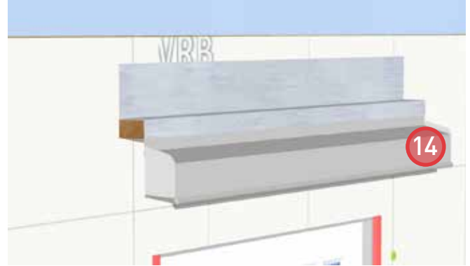
14. Install self-adhered membrane over the wood blocking. Extend the membrane onto the adjacent wall and the prefinished metal flashing.
