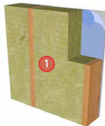
1. Typical 2x6 wood frame construction with ROXUL® COMFORTBATT® installed in the stud cavities.
