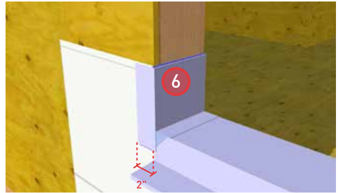
6. Install self-adhered membrane at sill corners, extending up the jamb to the height of the sheathing membrane. Finish the self-adhered membrane 2" onto the face of the wall.
