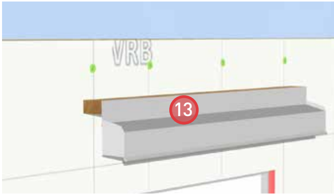
13. Install prefinished metal flashing above the swing door head. Block the flashing out beyond the plane of insulation using treated wood blocking.
