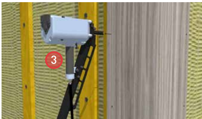
3. Install strapping as required to support the corner trim boards and cladding. Install corner trim boards.
