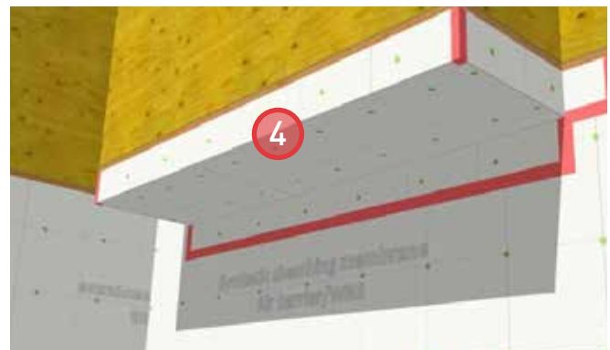
4. Install sheathing membrane along the cantilevered floor joists. Seal all leading edges with sheathing tape to maintain air barrier continuity. Fold corners on the upturn and seal the fold with sheathing tape.
