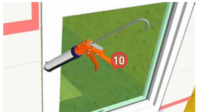
10. Install backer rod and sealant around the jamb and head of the window to aid in water diversion.
