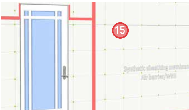
15. Install sheathing membrane to the rest of the wall. Seal the vertical leading edge with sheathing tape to maintain air barrier continuity.
