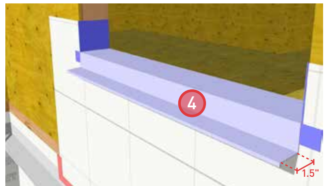
4. Install secondary self-adhered sill membrane to aid in diverting water outboard of the exterior insulation. Leave the facer on the unsupported portion of the membrane until insulation is installed.
