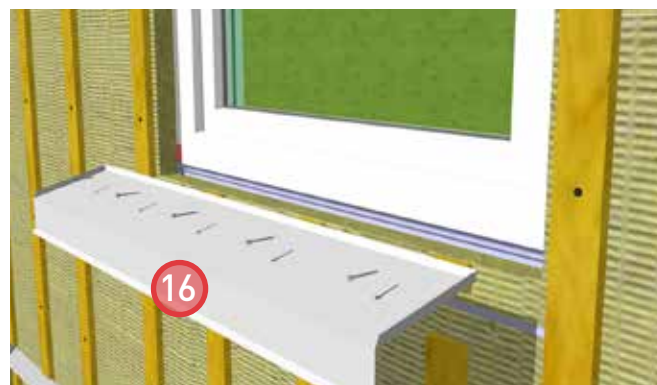
16. Install prefinished metal sill flashing. Refer to window manufacturer's specifications for more information.
