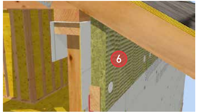
6. Install ROXUL® COMFORTBOARD™ 80 and secure with recommended fasteners.
