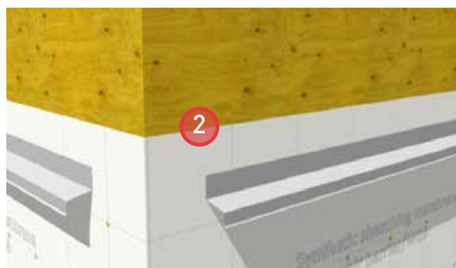
2. Install sheathing membrane and flashing.
