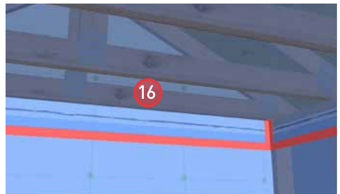
16. Install poly to the underside of the roof framing and fasten with staples at the sealant bead to complete the air seal. Seal the leading edge with sheathing tape.
