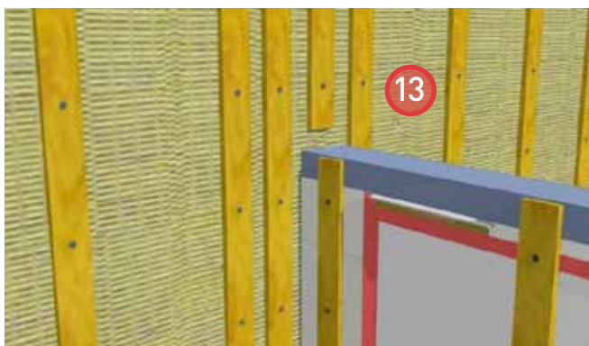
13. Install ROXUL® COMFORTBOARD™ 80 and secure in place with strapping. Provide bugscreens at the top and bottom of the strapping.
