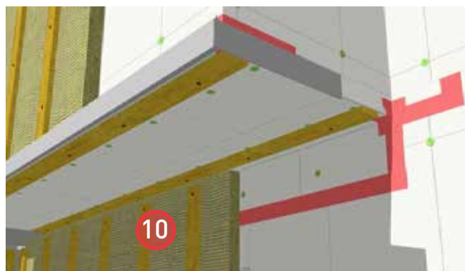
10. Install ROXUL® COMFORTBOARD™ 80 and strapping. Provide bugscreens at the top and bottom of the strapping. Optional: Install ROXUL® COMFORTBOARD™ 80 and strapping to the underside of the cantilevered floor.
