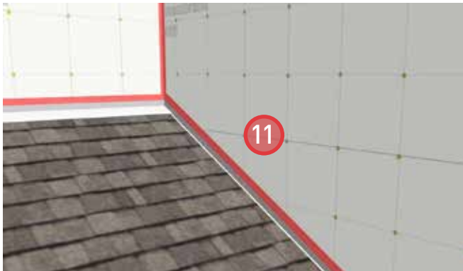
11. Seal all edges of the sheathing membrane with sheathing tape.
