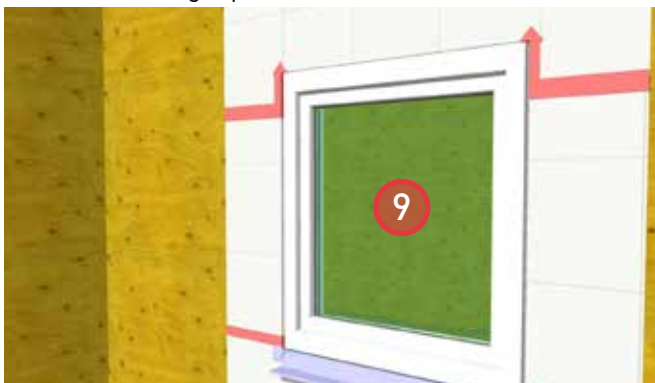
9. Install and structurally attach window per manufacturer's specifications.
