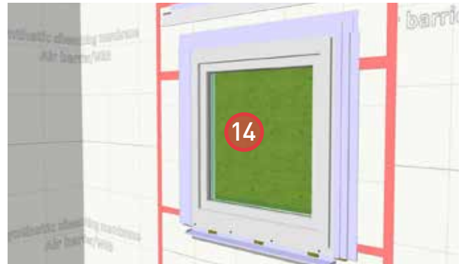
14. Install sheathing membrane. Ensure positive laps over all other layers. Seal the leading edge with sheathing tape.
