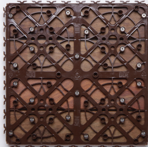
12"x12" Deck Tile (Bottom side)
