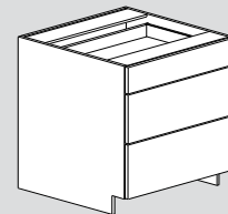
3 DRAWER BANK 34-3/4"H X 23-5/8"
